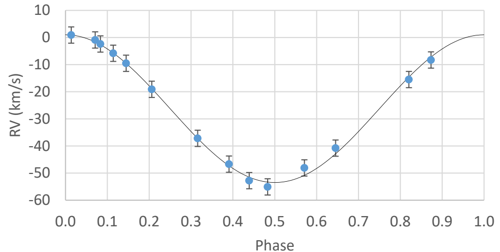
T CrB radial velocity (2016)
